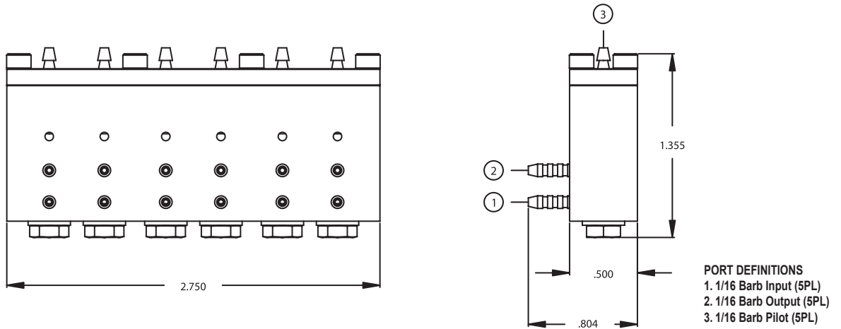
Part # 206890 Logic Valve
