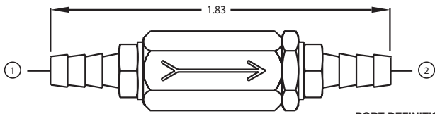
PORT DEFINITIONS 1. 1/8 Barb Input 2. 1/8 Barb Output
